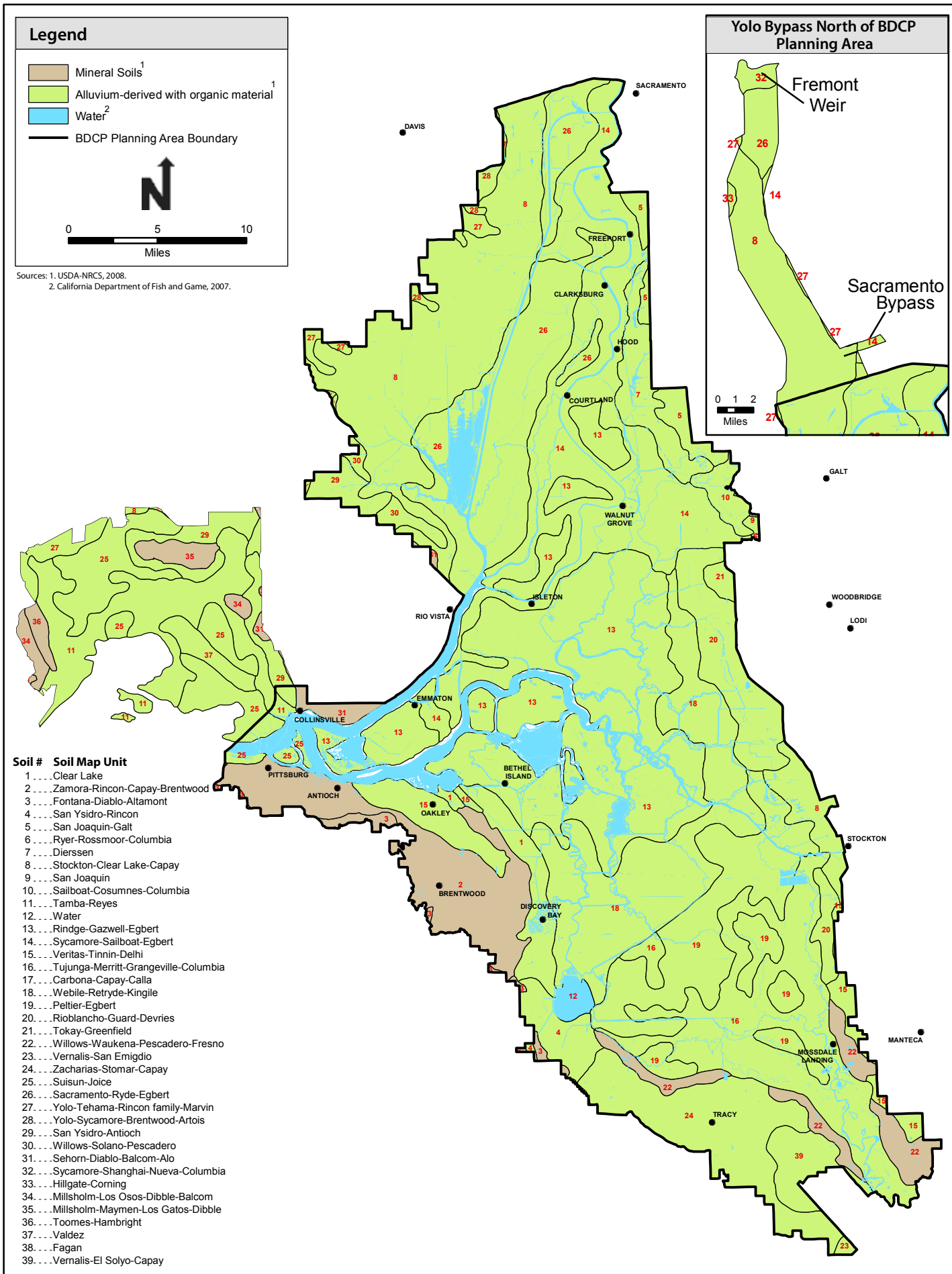
Figure 2.4. Soil Types of the BDCP Planning Area, Suisun Marsh, and Upper Yolo Bypass
