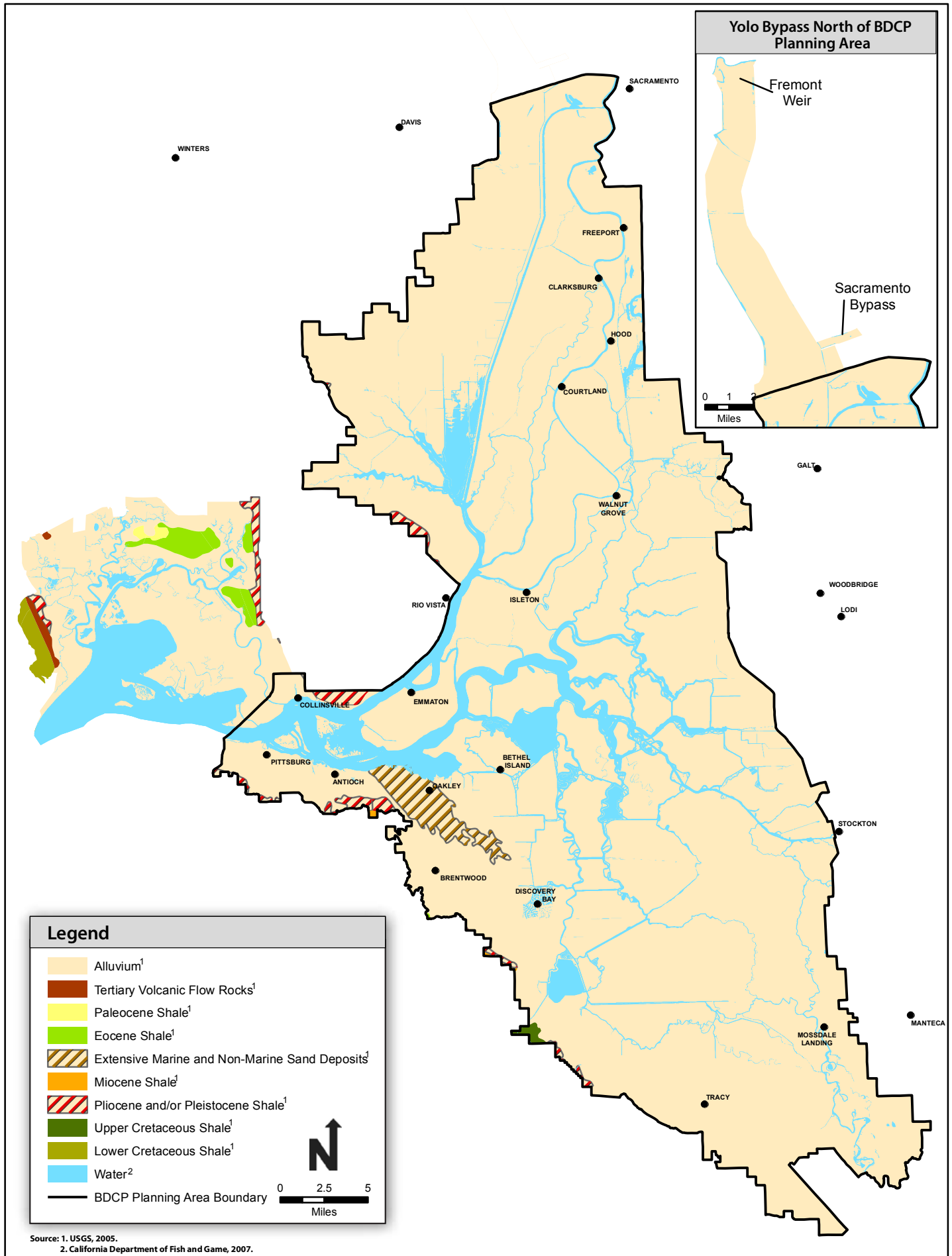
Figure 2.3. Geology of the BDCP Planning Area, Suisun Marsh, and Upper Yolo Bypass
