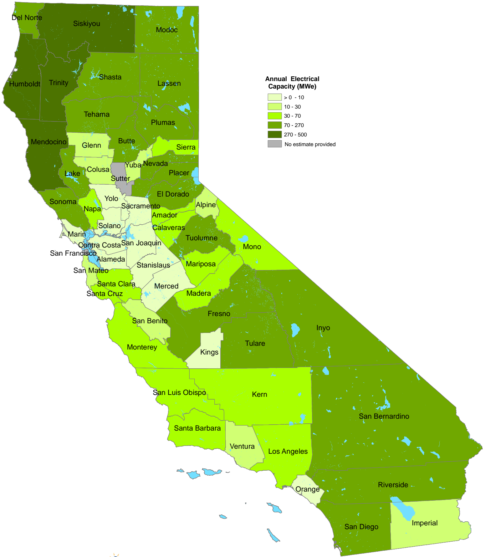
Figure 10a. Annual Electrical Capacity (MWe) from Gross potential, by county.
